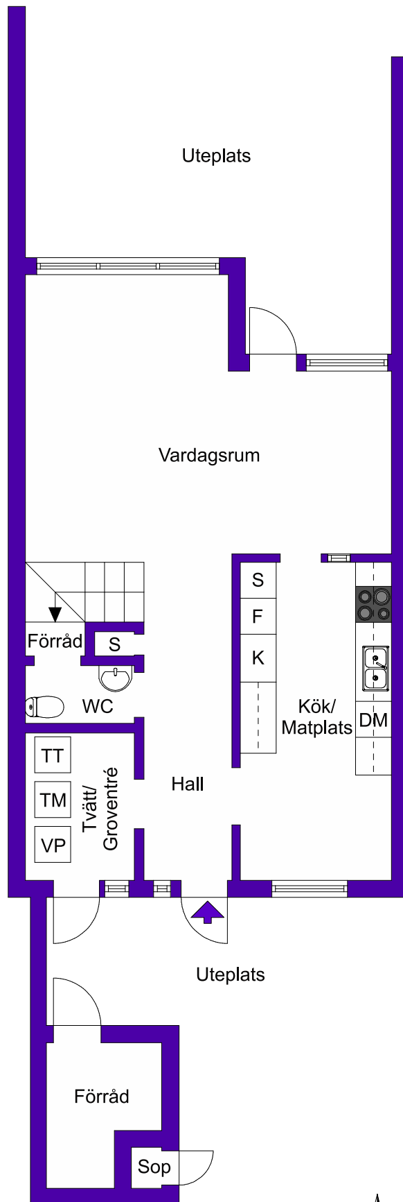
Bottenplan
